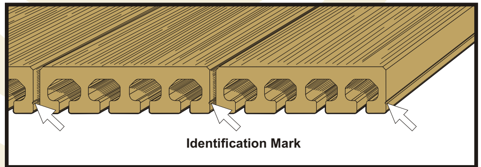
Install all decking with Identification Marks on the same side.
